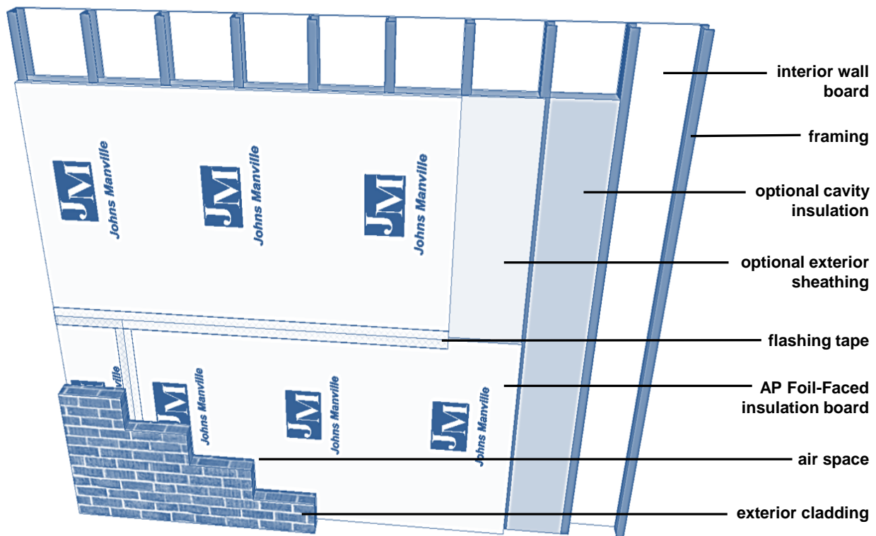
Figure 1. JM Continuous Insulation Wall System
